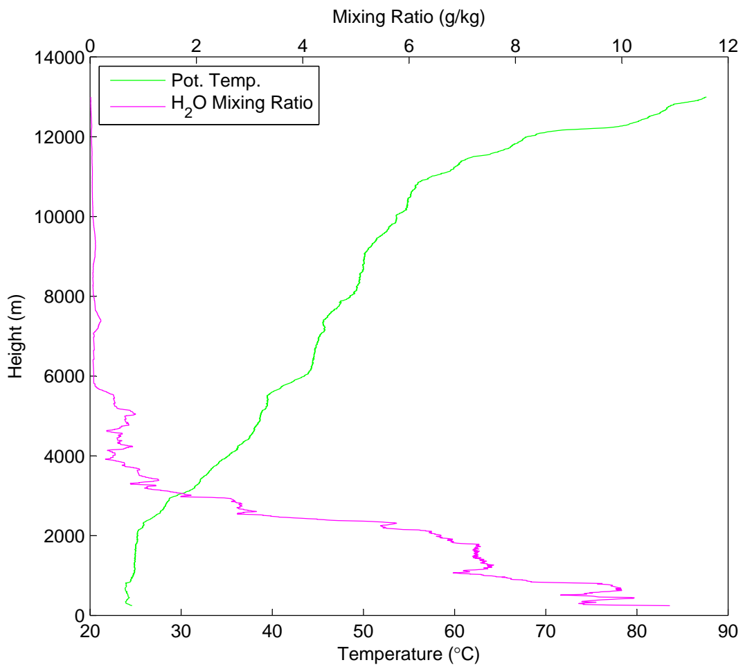
Potential Temperature & Water Vapor Mixing Ratio vs Height on June 30 at 15:23 UTC
