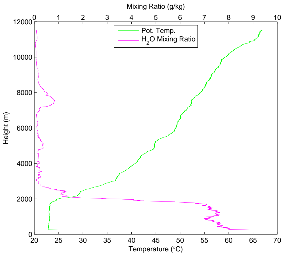
Potential Temperature & Water Vapor Mixing Ratio vs Height on July 03 at 18:52 UTC
