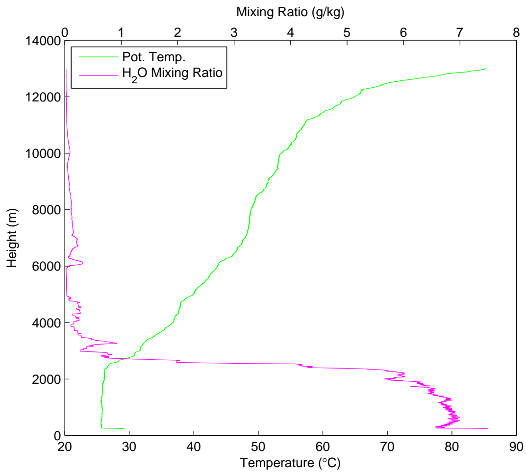
Potential Temperature & Water Vapor Mixing vs Height Ratio vs Height on June 30 at 19:11 UTC
