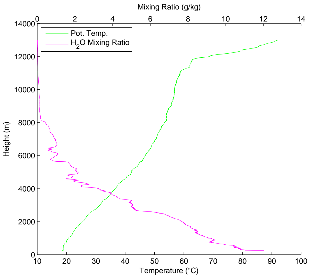
Potential Temperature & Water Vapor Mixing Ratio vs Height on June 29 at 15:14 UTC
