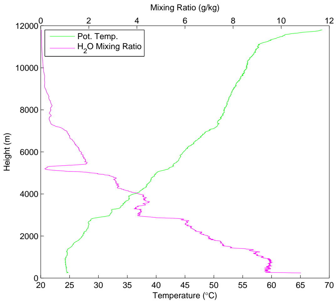
Potential Temperature & Water Vapor Mixing Ratio vs Height on June 29 at 19:55 UTC
