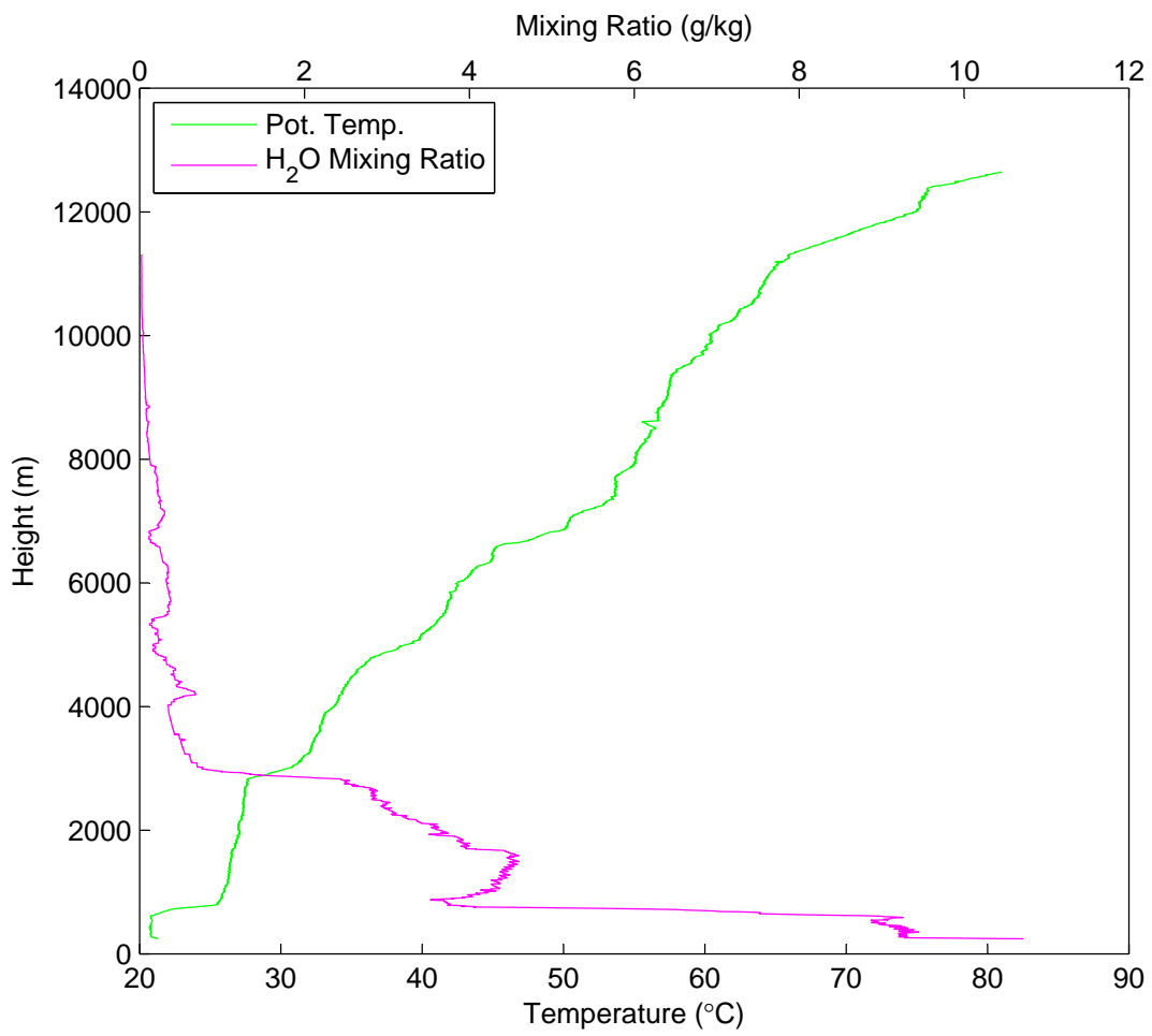
Potential Temperature & Water Vapor Mixing Ratio vs Height on June 28 at 14:00 UTC
