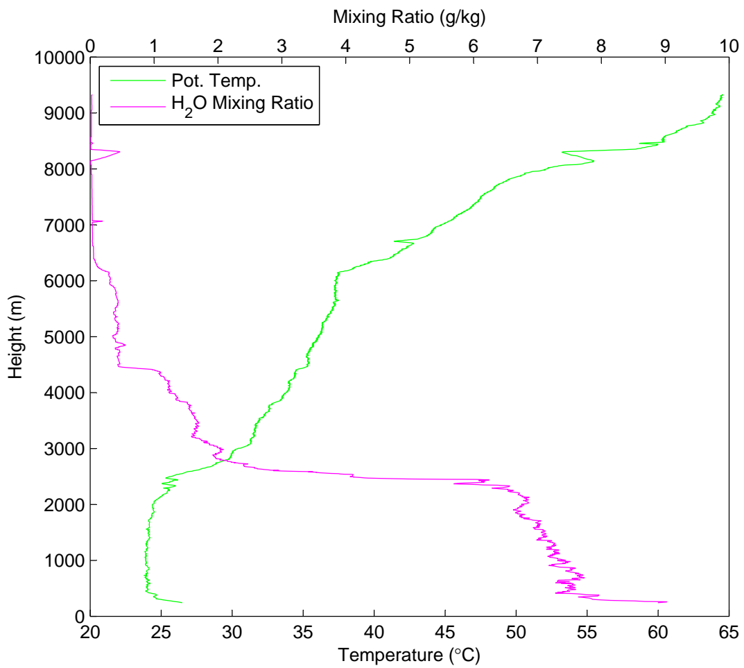
Potential Temperature & Water Vapor Mixing Ratio vs Height on June 28 at 19:06 UTC
