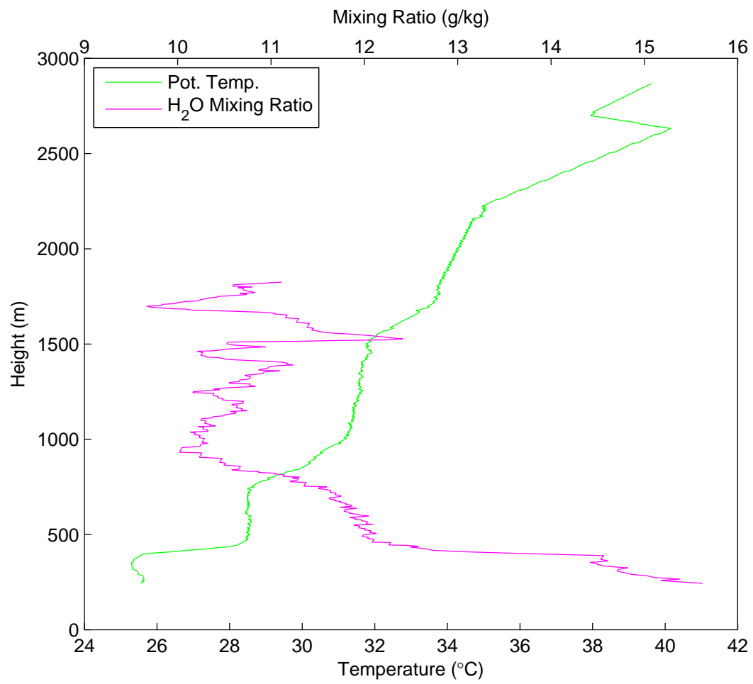
Potential Temperature & Water Vapor Mixing Ratio vs Height on June 26 at 14:59 UTC
