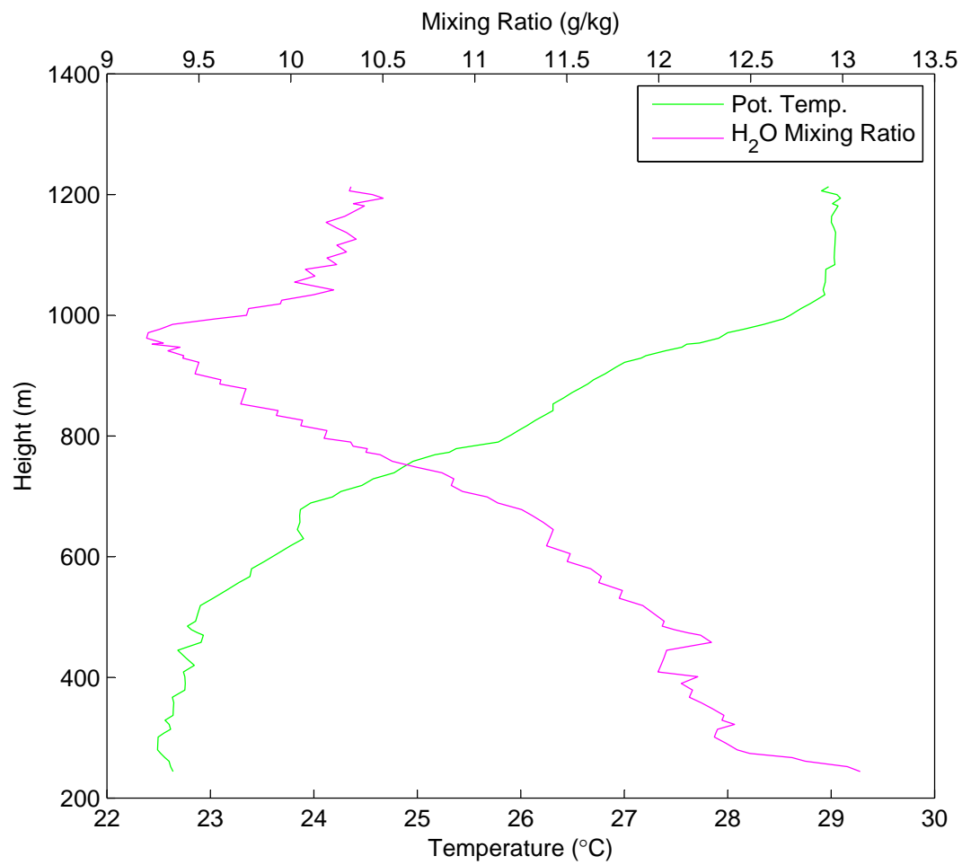
Potential Temperature & Water Vapor Mixing Ratio vs Height on June 26 at 18:50 UTC
