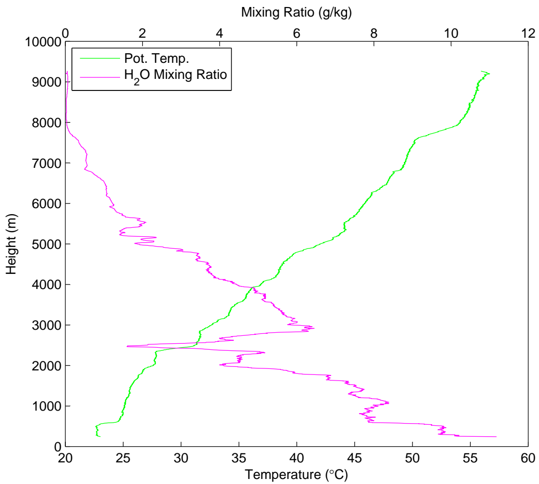
Potential Temperature & Water Vapor Mixing Ratio vs Height on June 24 at 13:47 UTC
