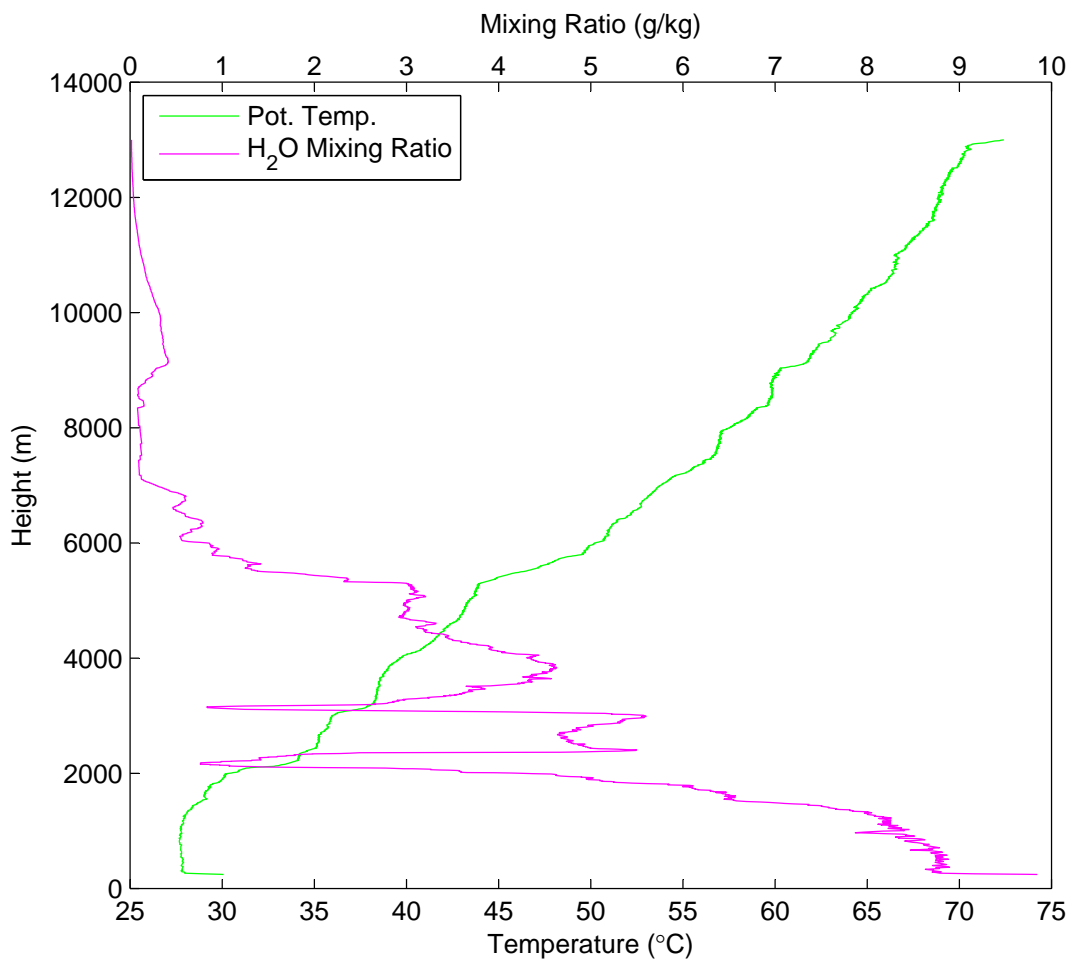
Potential Temperature & Water Vapor Mixing Ratio vs Height on June 24 at 18:59 UTC
