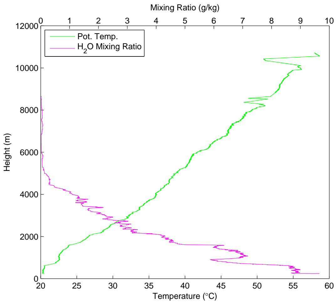
Potential Temperature & Water Vapor Mixing Ratio vs Height on June 23 at 14:03 UTC
