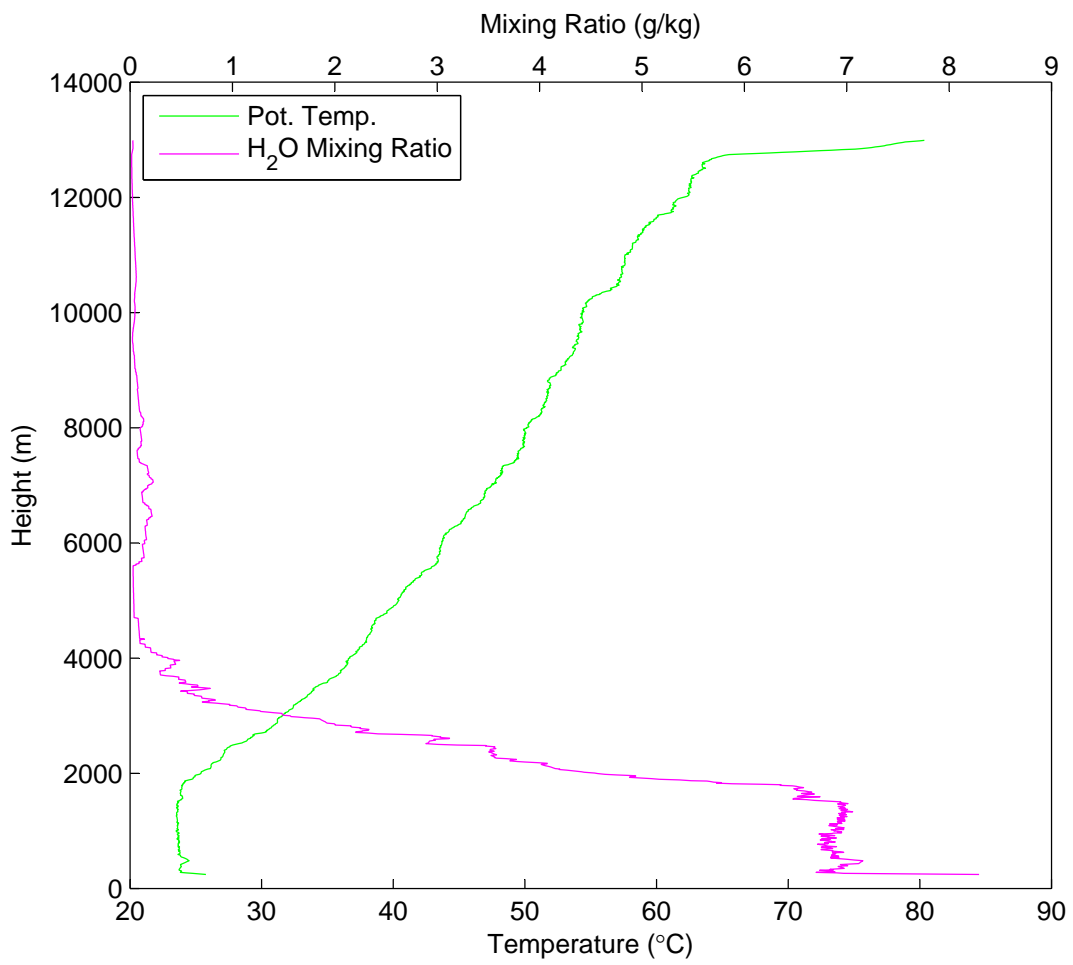
Potential Temperature & Water Vapor Mixing Ratio vs Height on June 23 at 19:08 UTC
