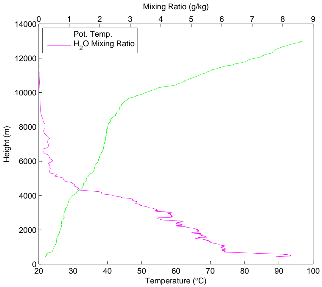
Potential Temperature & Water Vapor Mixing Ratio vs Height on June 22 at 14:06 UTC
