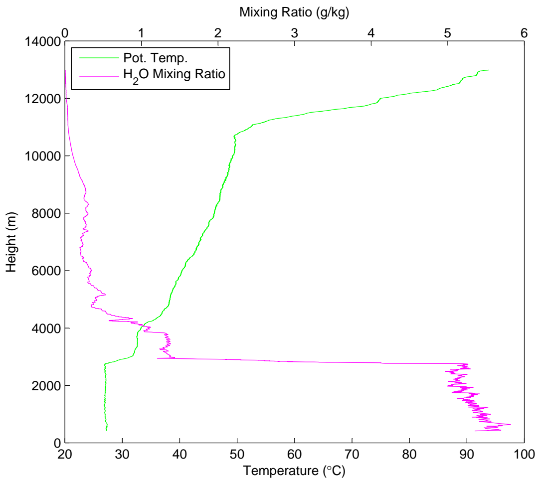
Potential Temperature & Water Vapor Mixing Ratio vs Height on June 21 at 18:51 UTC
