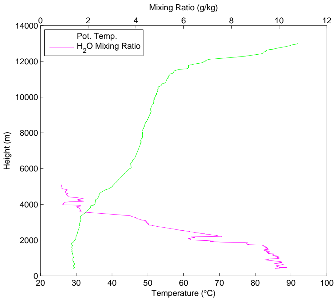
Potential Temperature & Water Vapor Mixing Ratio vs Height on June 20 at 19:11 UTC
