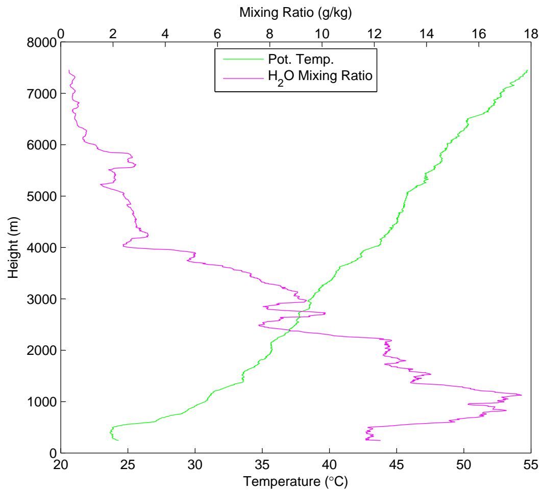
Potential Temperature & Water Vapor Mixing Ratio vs Height on July 06 at 13:55 UTC
