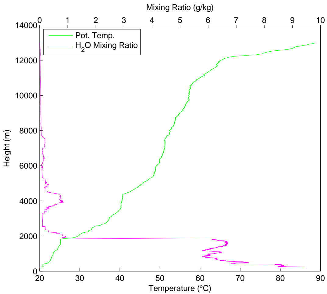
Potential Temperature & Water Vapor Mixing Ratio vs Height on July 05 at 13:55 UTC
