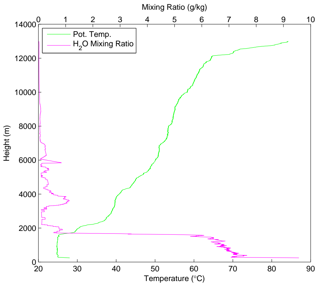
Potential Temperature & Water Vapor Mixing Ratio vs Height on July 05 at 18:31 UTC
