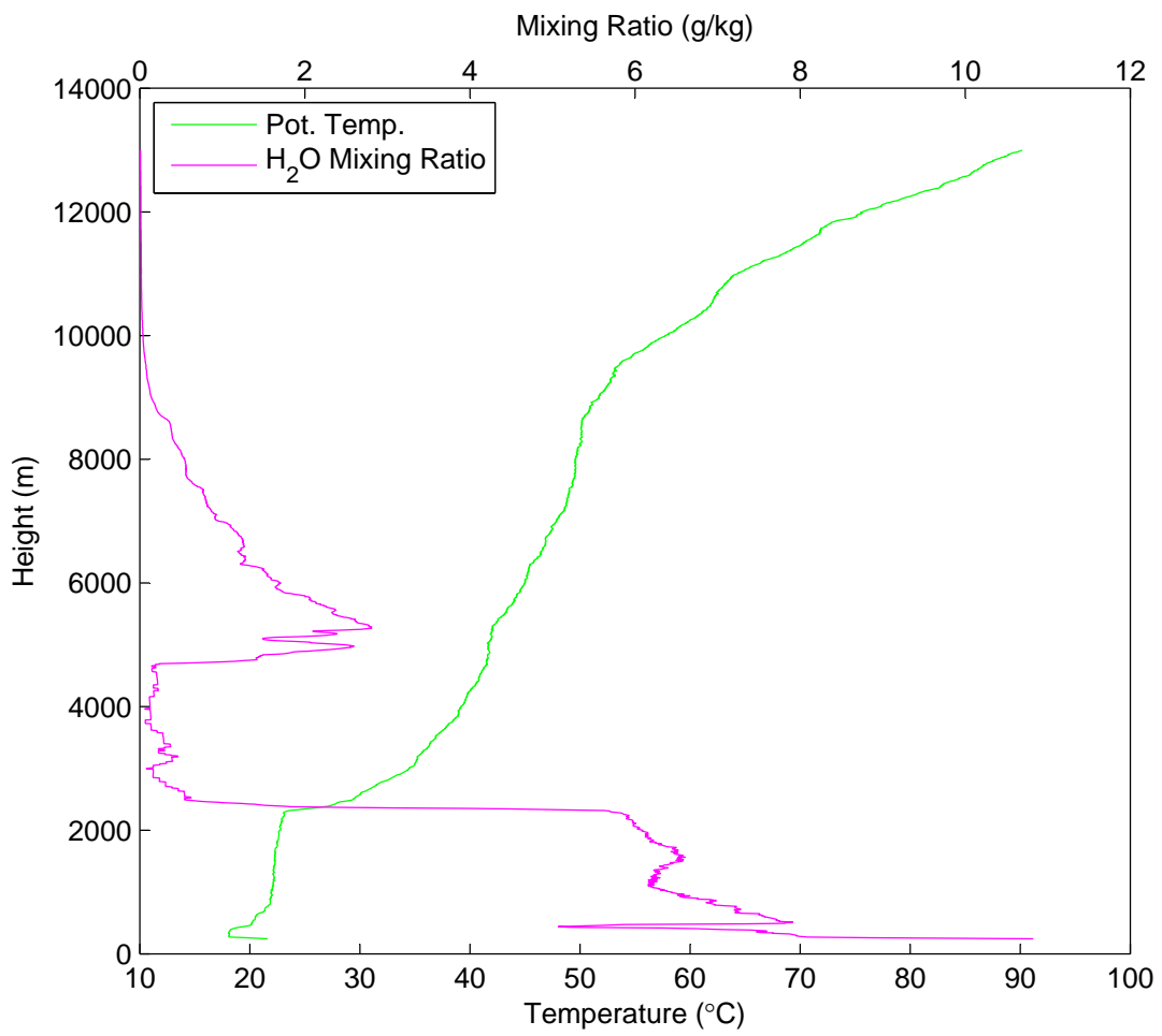
Potential Temperature & Water Vapor Mixing Ratio vs Height on July 04 at 13:58 UTC
