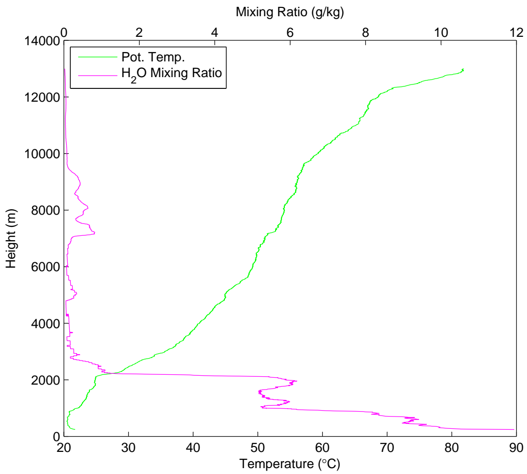
Potential Temperature & Water Vapor Mixing Ratio vs Height on July 03 at 15:02 UTC
