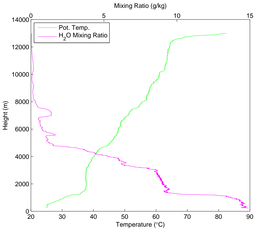
Potential Temperature & Water Vapor Mixing Ratio vs Height on July 02 at 13:52 UTC
