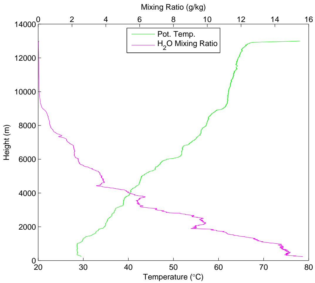
Potential Temperature & Water Vapor Mixing Ratio vs Height on July 02 at 18:47 UTC
