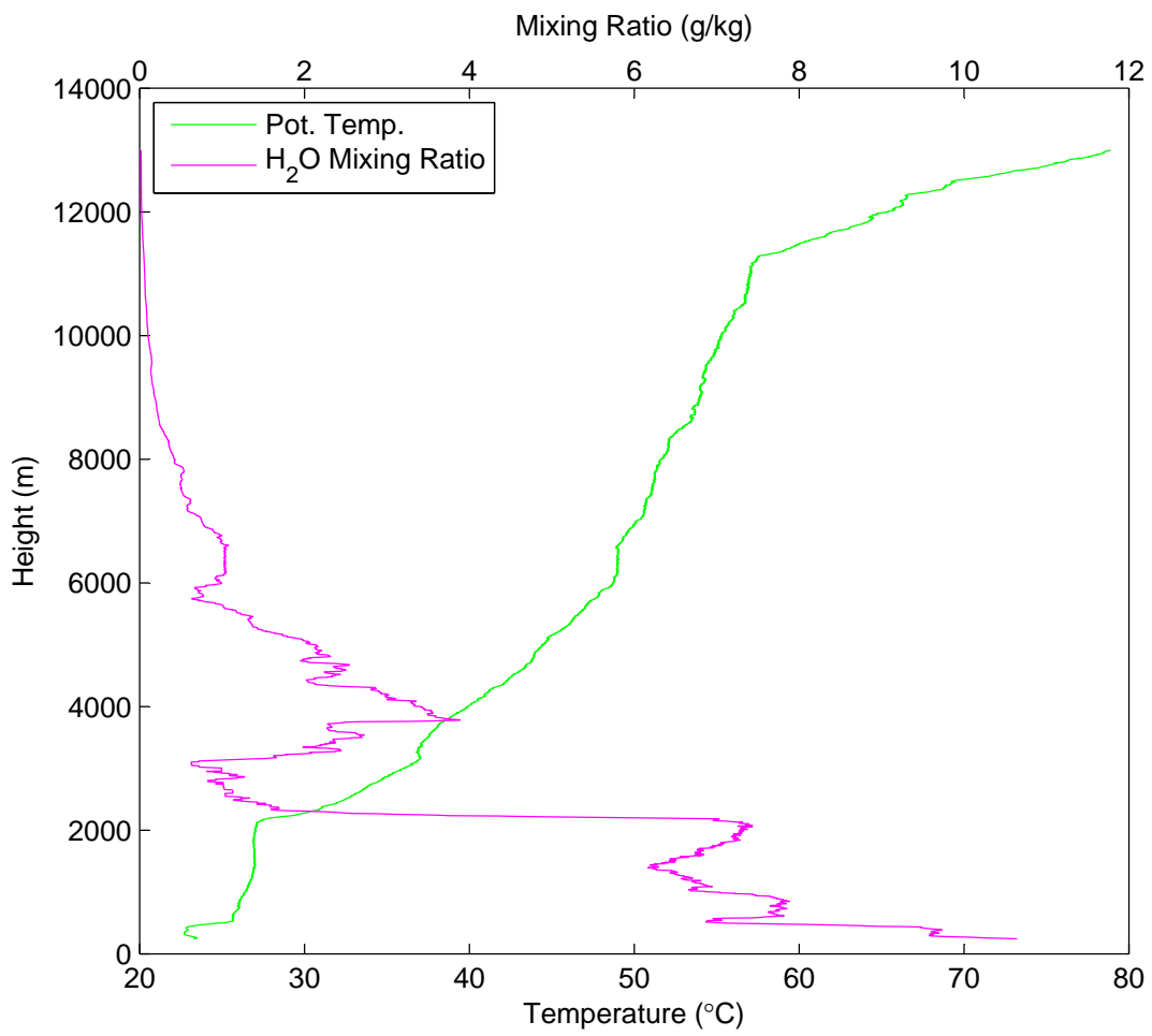
Potential Temperature & Water Vapor Mixing Ratio vs Height on July 01 at 14:32 UTC
