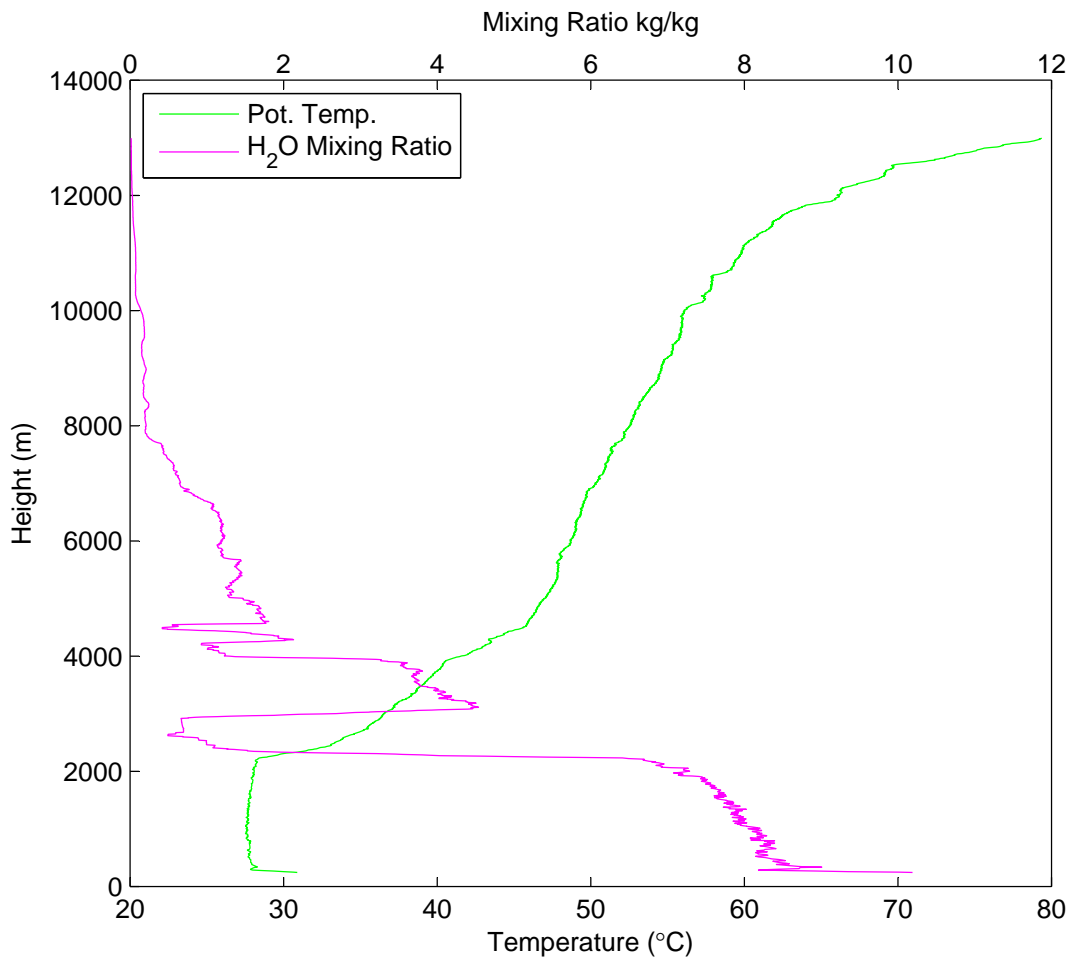
Potential Temperature & Water Vapor Mixing Ratio vs Height on July 01 at 18:53 UTC
